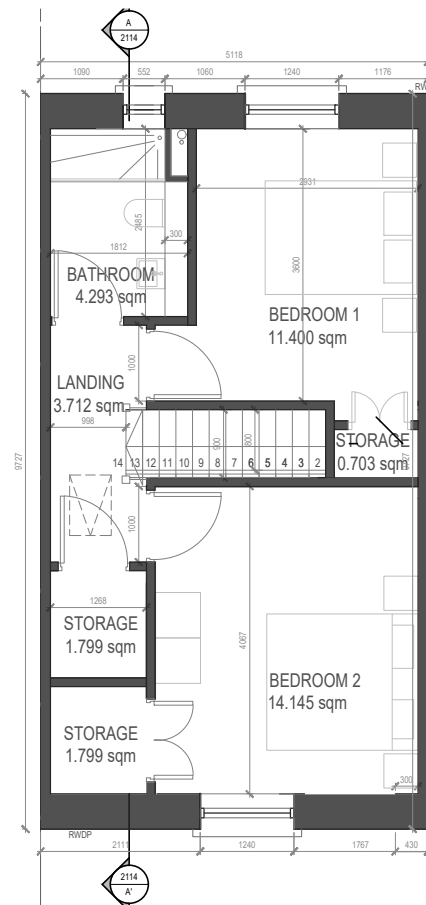
06 FIRST FLOOR PLAN
